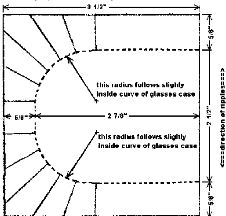
diner body top and bottom half plan
